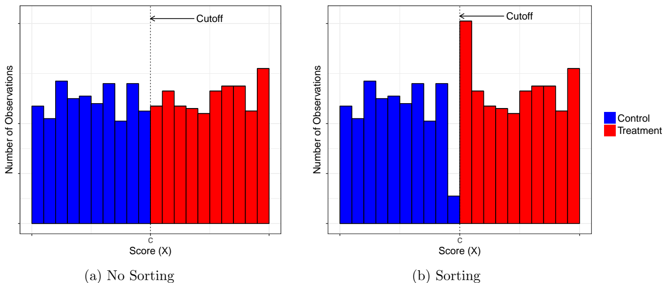
Figure 18: Histogram of Score
